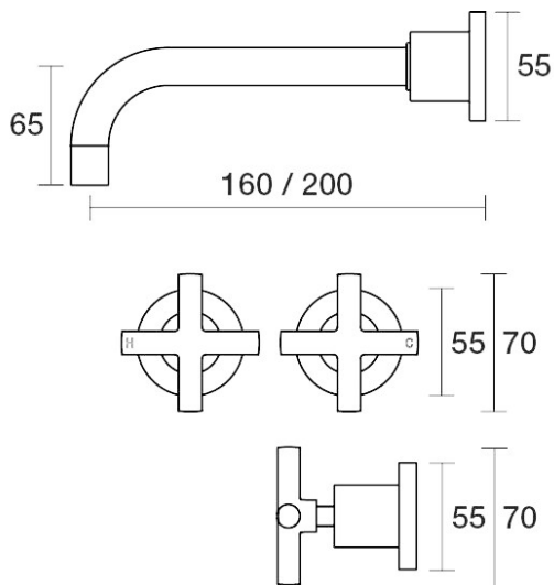
Portsea Wall Bath Set 160mm Outlet Ceramic Disc B29.021.2.68 - Autumn Bronze
