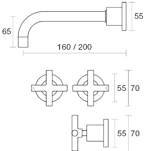
Portsea Wall Bath Set 200mm Outlet B29.022.1.01 - Chrome
