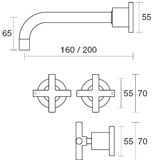
Portsea Wall Bath Set 200mm Outlet Ceramic Disc B29.022.2.12 - 23k Brushed Gold
