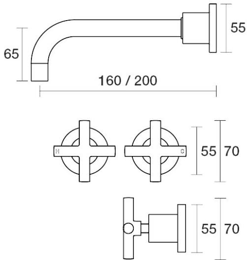
Portsea Wall Bath Set 200mm Outlet Ceramic Disc B29.022.2.26 - Black Sapphire
