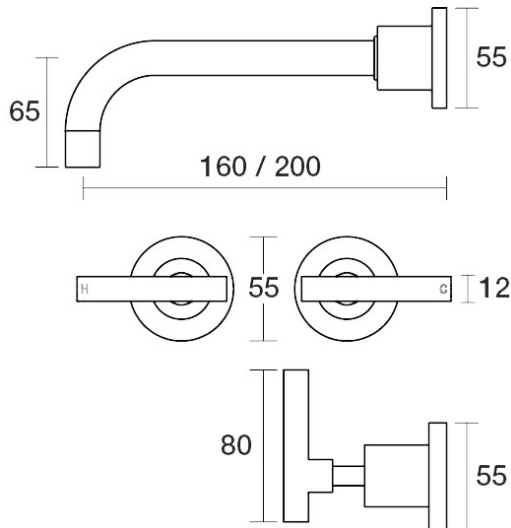
Portsea Wall Bath Set 200mm Outlet Lever Ceramic Disc B29.022.3.41 - Brushed Brass
