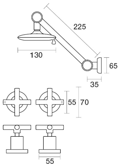
Portsea Shower Set Adjustable Arm B29.031.1.23 - Gunmetal
