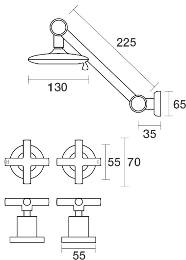
Portsea Shower Set Adjustable Arm B29.031.1.47 - Luminick
