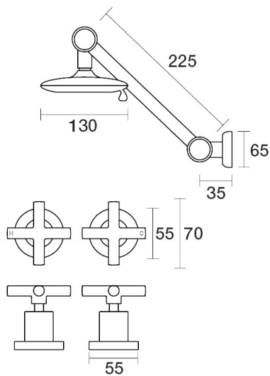
Portsea Shower Set Adjustable Arm B29.031.1.54 - Volcanic Grey
