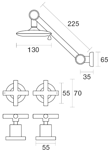
Portsea Shower Set Adjustable Arm Ceramic Disc B29.031.2.01 - Chrome
