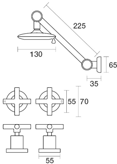
Portsea Shower Set Adjustable Arm Ceramic Disc B29.031.2.11 - 23k Gold
