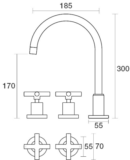
Portsea Sink Set Hob Swivel Ceramic Disc B29.051.2.23 - Gunmetal
