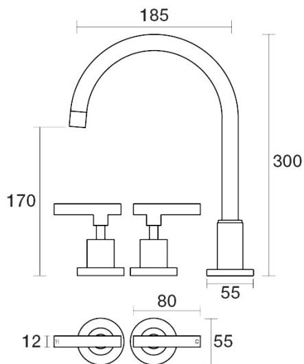
Portsea Sink Set Hob Swivel Lever Ceramic Disc B29.051.3.43 - Brass
