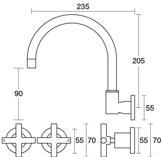
Portsea Sink Set Wall Swivel B29.052.1.44 - Antique Copper
