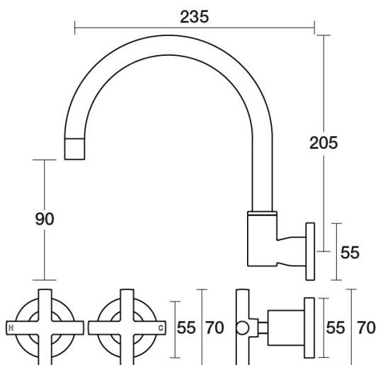
Portsea Sink Set Wall Swivel Ceramic Disc B29.052.2.42 - Brushed Copper
