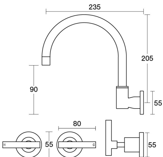
Portsea Sink Set Wall Swivel Lever Ceramic Disc B29.052.3.21 - Brushed Rose Gold
