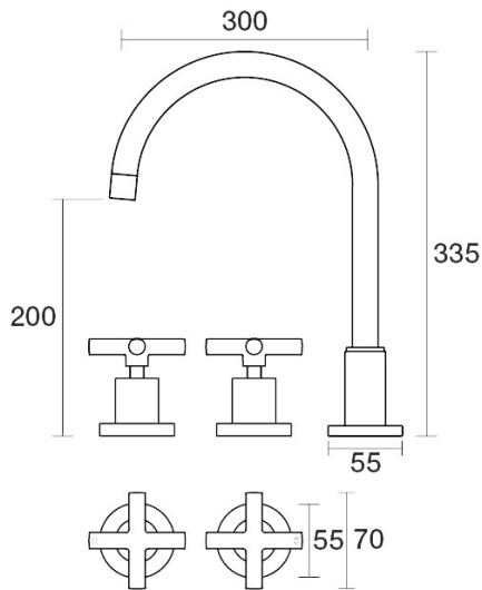
Portsea Sink Set XL Hob Swivel B29.053.1.12 - 23k Brushed Gold
