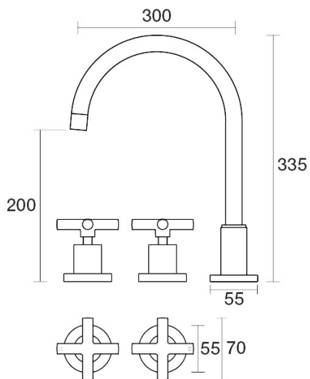
Portsea Sink Set XL Hob Swivel B29.053.1.23 - Gunmetal
