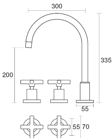
Portsea Sink Set XL Hob Swivel B29.053.1.48 - Copper
