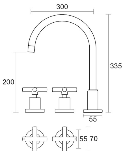
Portsea Sink Set XL Hob Swivel B29.053.1.67 - Vintage Brass
