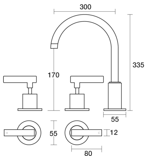
Portsea Sink Set XL Hob Swivel Lever Ceramic Disc 29.053.3.27 - Satin Pearl
