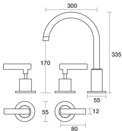
Portsea Sink Set XL Hob Swivel Lever Ceramic Disc 29053.3.42 - Brushed Copper
