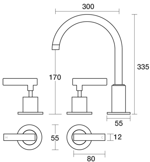
Portsea Sink Set XL Hob Swivel Lever Ceramic 29053.3.44 - Antique Copper
