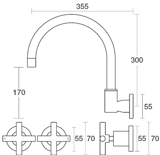
Portsea Sink Set XL Wall Swivel Ceramic Disc B29.054.2.21 - Brushed Rose Gold
