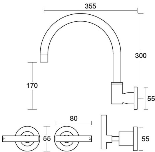
Portsea Sink Set XL Wall Swivel Lever Ceramic Disc 29054.3.01 - Chrome
