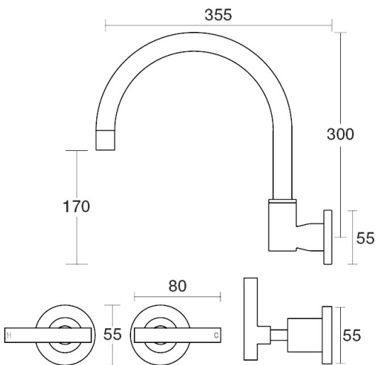
Portsea Sink Set XL Wall Swivel Lever Ceramic 29.054.3.43 - Brass
