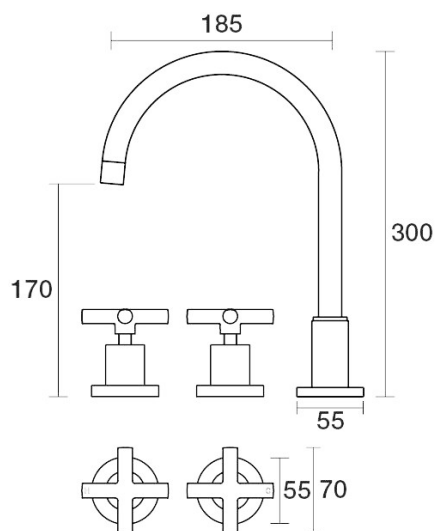
Portsea Spa Set Hob Swivel B29.061.1.23 - Gunmetal
