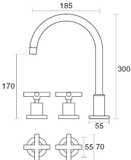
Portsea Spa Set Hob Swivel Ceramic Disc B29.061.2.40 - Rumbled Brass
