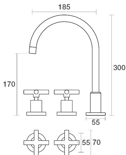
Portsea Spa Set Hob Swivel Ceramic Disc B29.061.2.47 - Luminick
