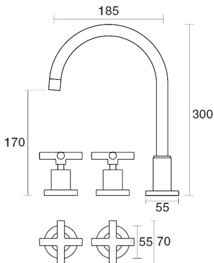
Portsea Spa Set Hob Swivel Ceramic Disc B29.061.2.67 - Vintage Brass
