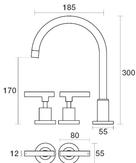
Portsea Spa Set Hob Swivel Lever Ceramic Disc B29.061.3.32 - Midnight Black
