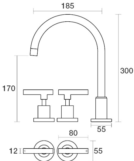
Portsea Spa Set Hob Swivel Lever Ceramic Disc B29.061.3.48 - Copper
