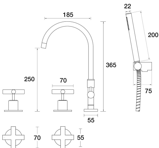
Portsea Spa Set Hob Swivel Divertor Set with Handshower & Bracket B29.061.4.27 - Satin Pearl
