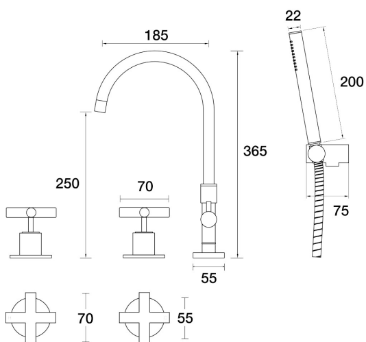
Portsea Spa Set Hob Swivel Divertor Set with Handshower & Bracket B29.061.4.54 - Volcanic Grey
