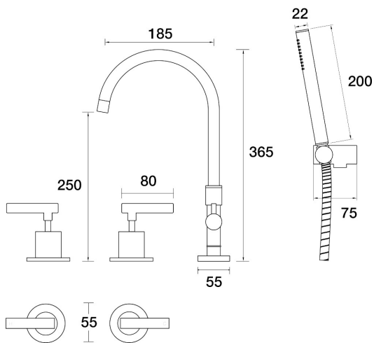
Portsea Spa Set Hob Swivel Divertor Set with Handshower & Bracket Lever Ceramic Disc B29.061.6.40 - Rumbled Brass
