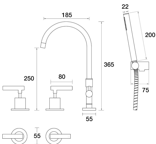
Portsea Spa Set Hob Swivel Divertor Set with Handshower & Bracket Lever Ceramic Disc B29.061.6.42 - Brushed Copper
