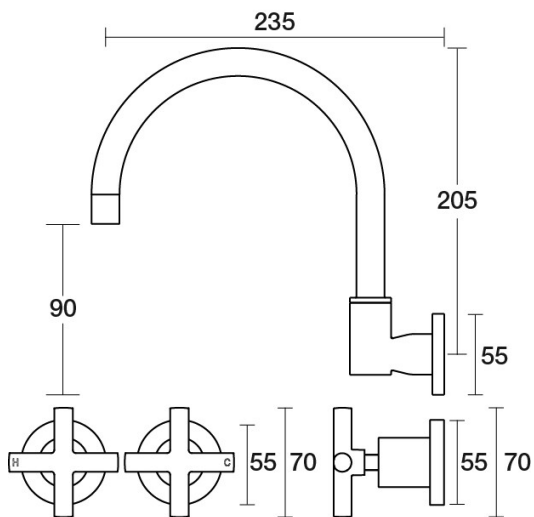
Portsea Spa Set Wall Swivel B29.062.1.02 - Brushed Chrome
