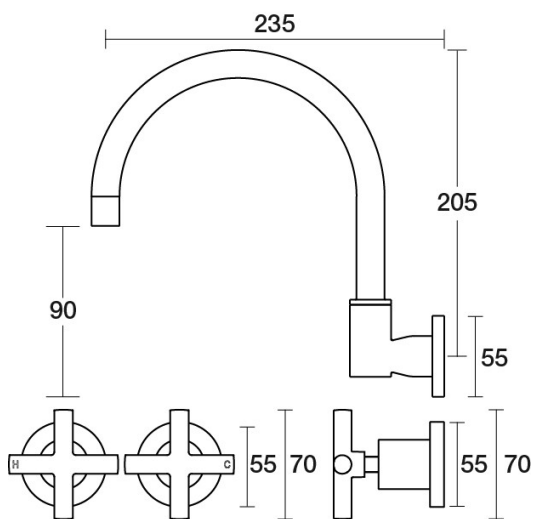
Portsea Spa Set Wall Swivel B29.062.1.52 - Burnished
