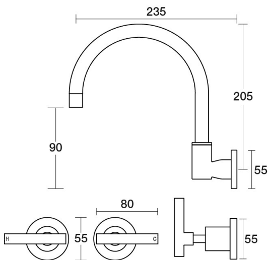
Portsea Spa Set Wall Swivel Lever Ceramic Disc B29.062.3.52 - Burnished
