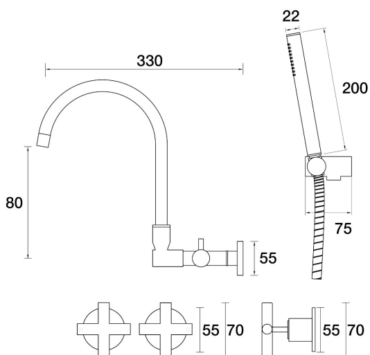
Portsea Spa Set Wall Swivel Divertor Set with Handshower & Bracket B29.062.4.39 - Antique Bronze
