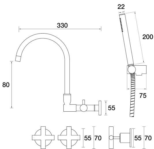
Portsea Spa Set Wall Swivel Divertor Set with Handshower & Bracket B29.062.4.54 - Volcanic Grey
