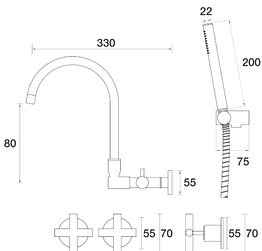
Portsea Spa Set Wall Swivel Divertor Set with Handshower & Bracket Ceramic Disc B29.062.5.01 - Chrome
