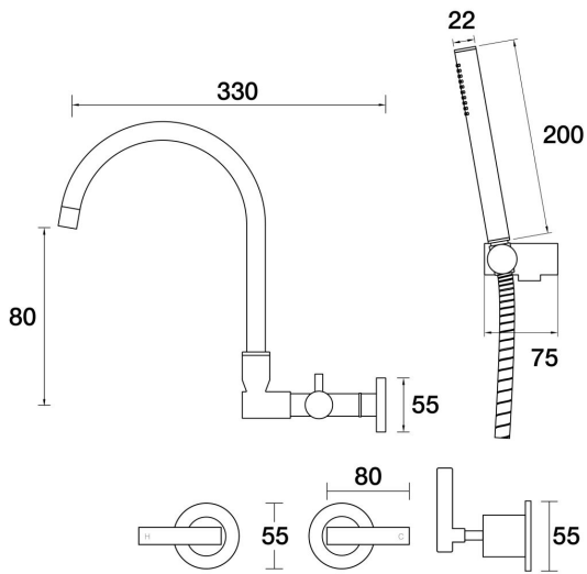
Portsea Spa Set Wall Swivel Divertor Set with Handshower & Bracket Lever Ceramic Disc B29.062.6.01 - Chrome
