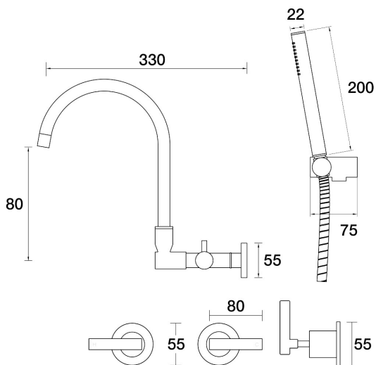
Portsea Spa Set Wall Swivel Divertor Set with Handshower & Bracket Lever Ceramic Disc B29.062.6.25 - Brushed Nickel
