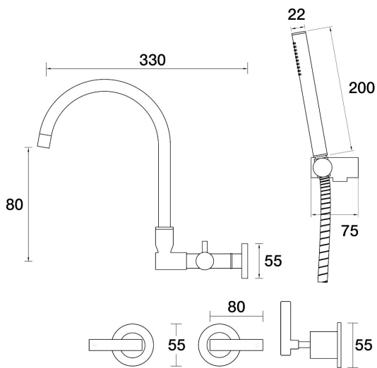
Portsea Spa Set Wall Swivel Divertor Set with Handshower & Bracket Lever Ceramic Disc B29.062.6.26 - Black Sapphire
