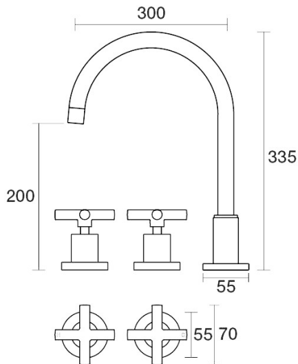
Portsea Spa Set XL Hob Swivel B29.063.1.19 - 23k Brushed Brass Gold
