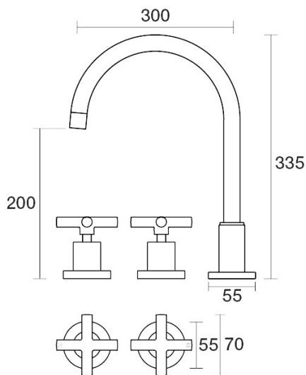
Portsea Spa Set XL Hob Swivel B29.063.1.32 - Midnight Black
