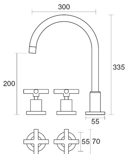
Portsea Spa Set XL Hob Swivel Ceramic Disc B29.063.2.02 - Brushed Chrome
