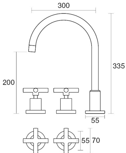
Portsea Spa Set XL Hob Swivel Ceramic Disc B29.063.2.21 - Brushed Rose Gold
