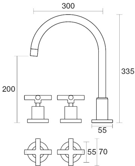
Portsea Spa Set XL Hob Swivel Ceramic Disc B29.063.2.45 - Native Brass
