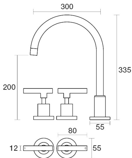
Portsea Spa Set XL Hob Swivel Lever Ceramic Disc B29.063.3.54 - Volcanic Grey
